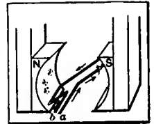
Fig. 7—Illustrating the direction of the current when the armature takes up the illustrated position. Current flowing from a to b.
